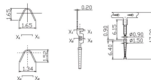
0.76 Crimp Pin Female Terminal PART No.HDBC-FT-L
